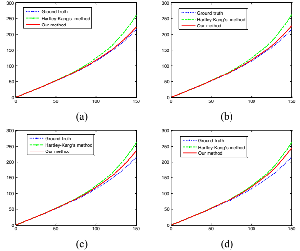
Fig. 2. Comparisons between algorithms of recovering radial distortion function with respect to different noise levels. These graphs of radial distortion correction r^u versus radial position r^d using grid points from a single image as shown in Fig. 1b. The number labels are all in pixels. (a) noise level \sigma = 0.25 . (b) \sigma = 0.5 (c) \sigma = 0.75 . (d) \sigma = 1 .
